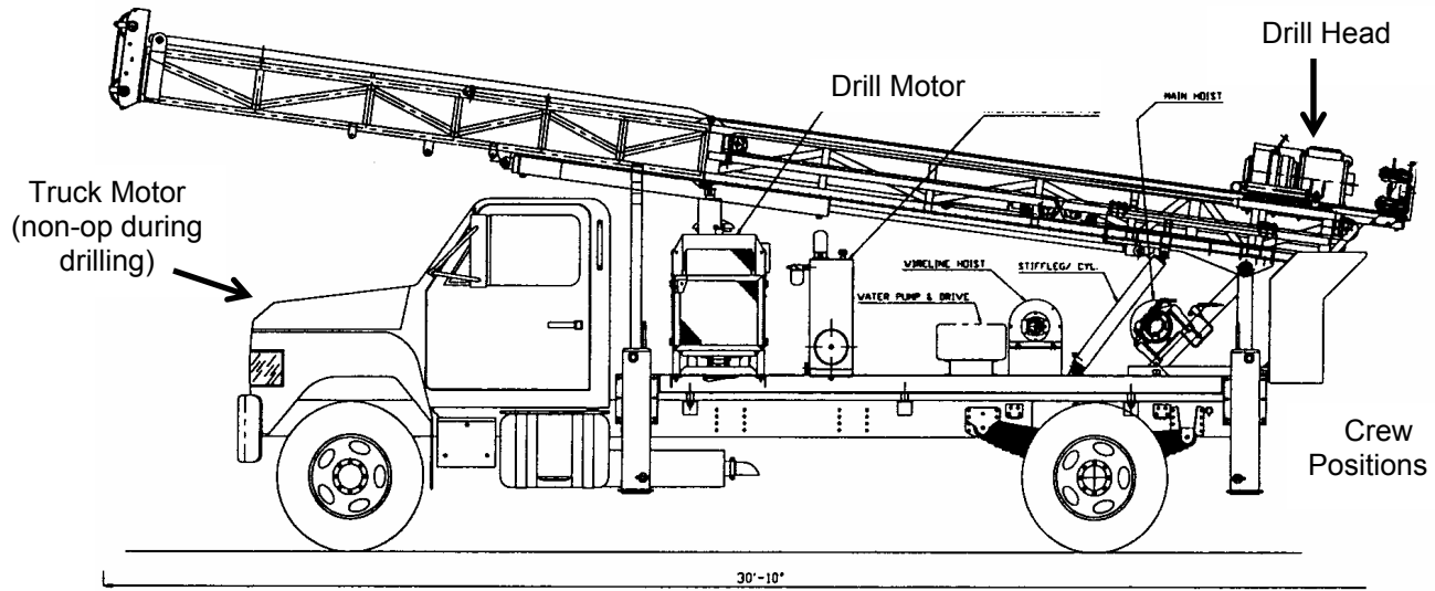
Figure 2 - Side View of CS1500 Core Drill Rig with Noise Sources Noted
